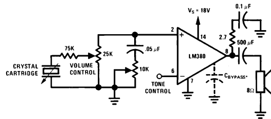
Phono Amplifier
