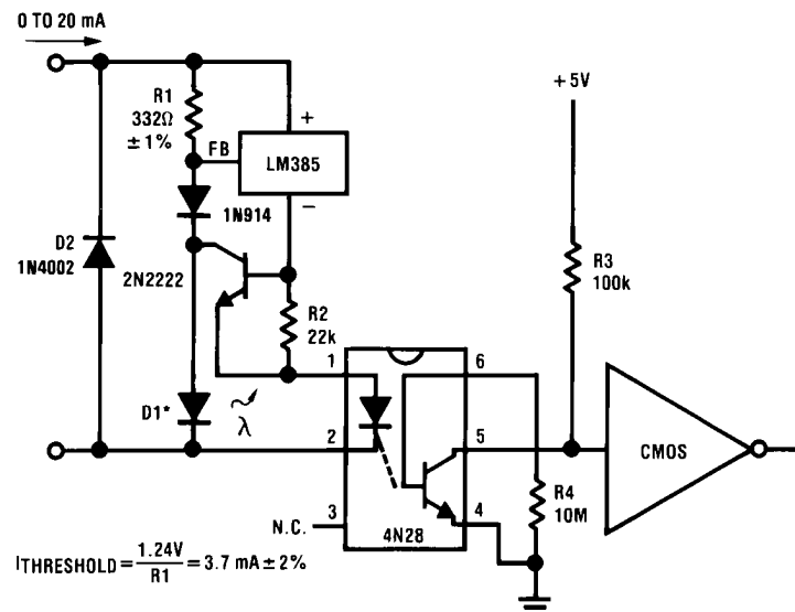
Precision Floating Current Detector
