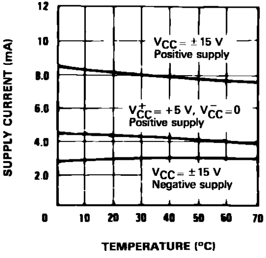
SUPPLY CURRENT
