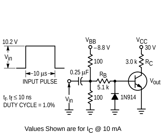
Figure 6. Switching Time Test Circuit
