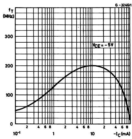
Transition Frequency.
